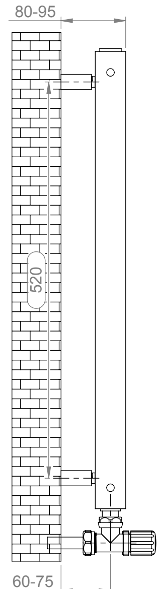
Side View
