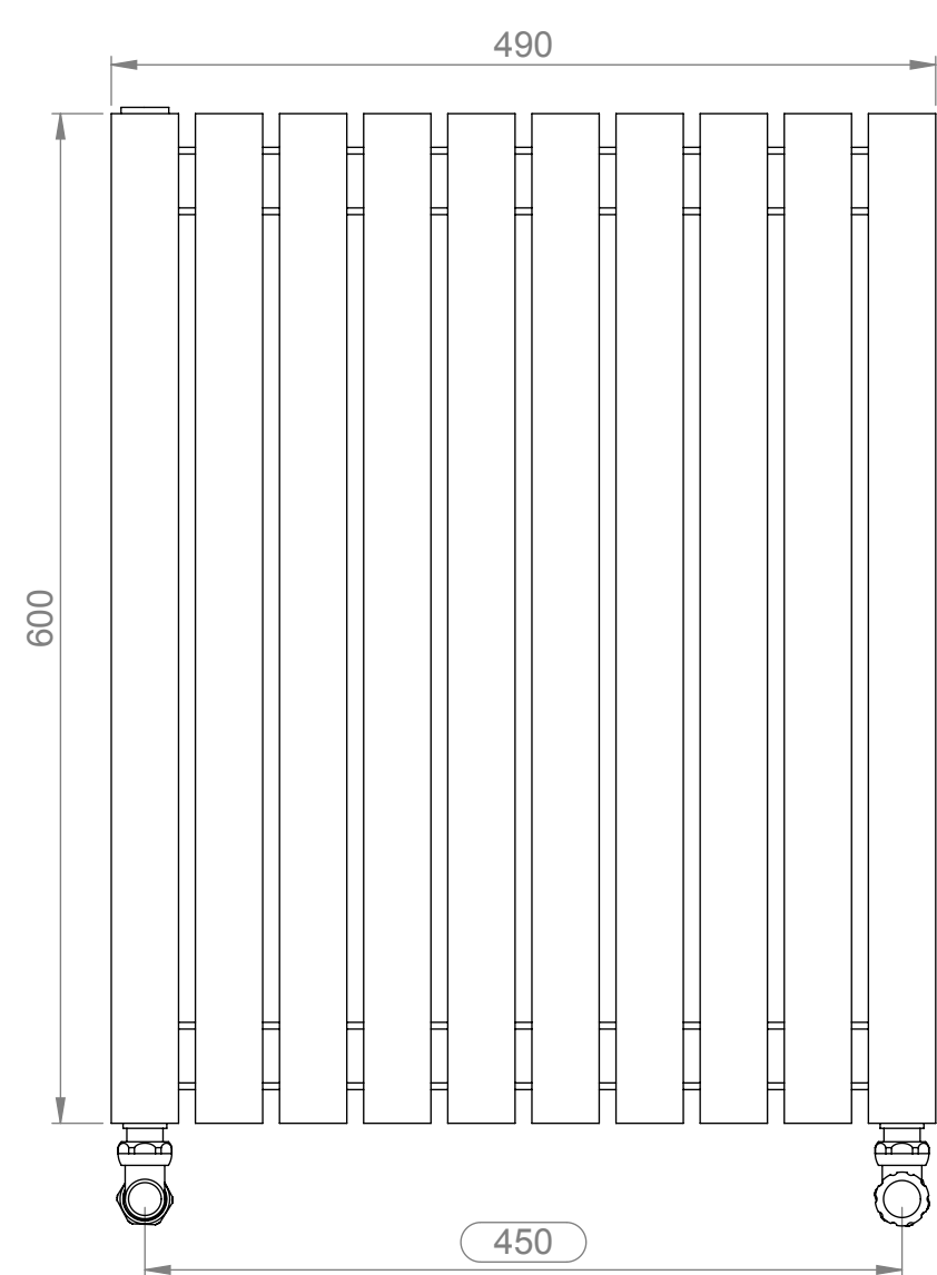
Front View
