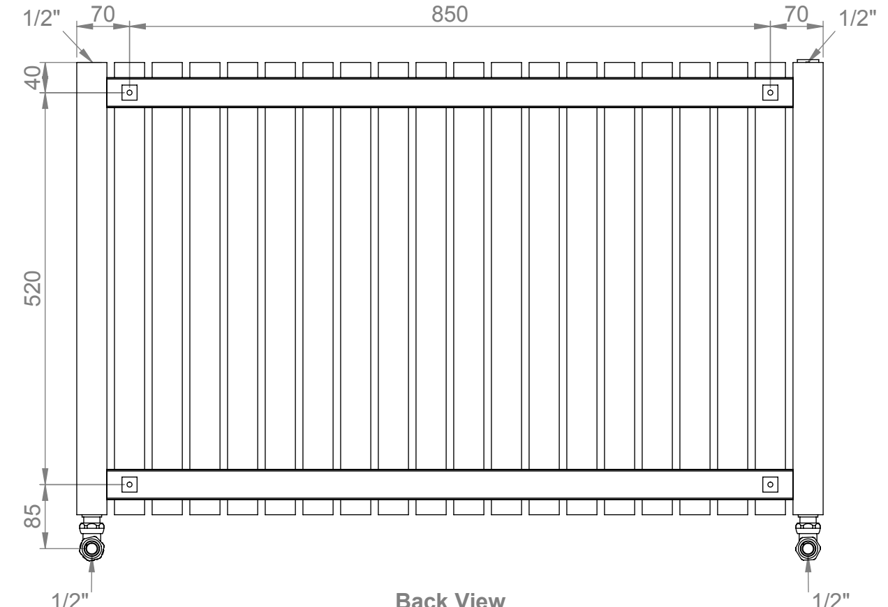
Back View
