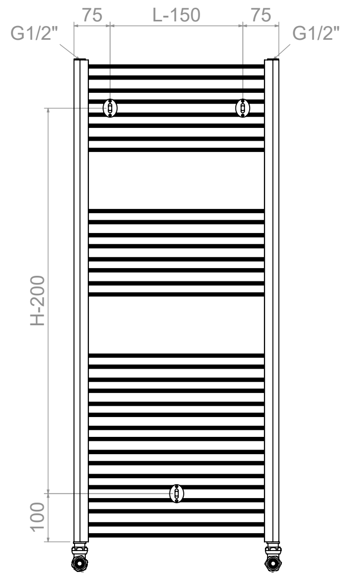
Back View
