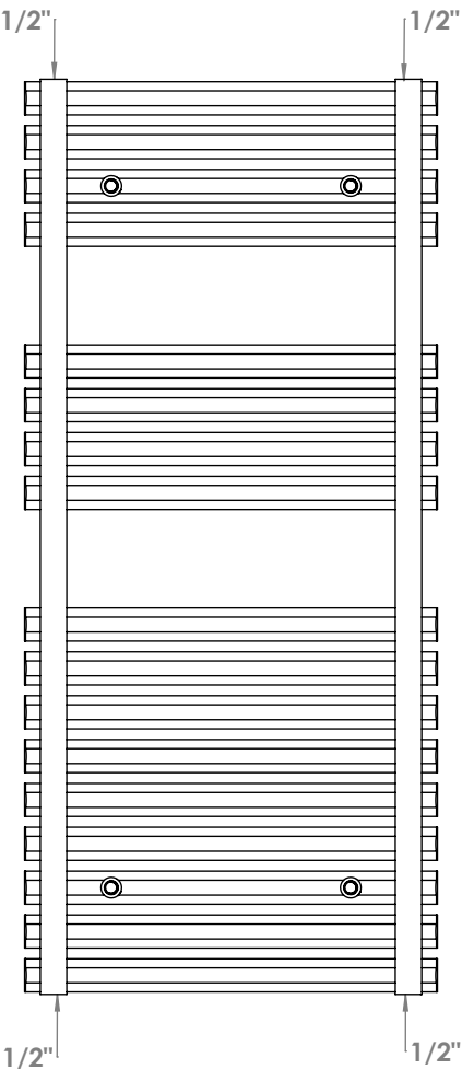
Back View
