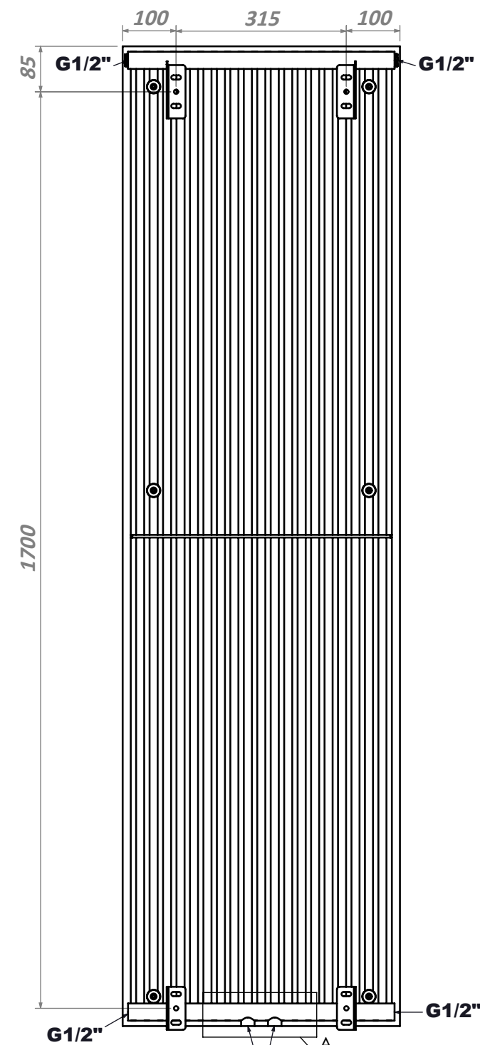
Back View
