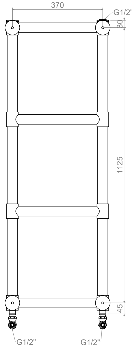
Back View
