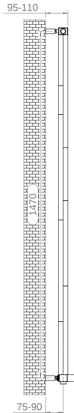
Side View
