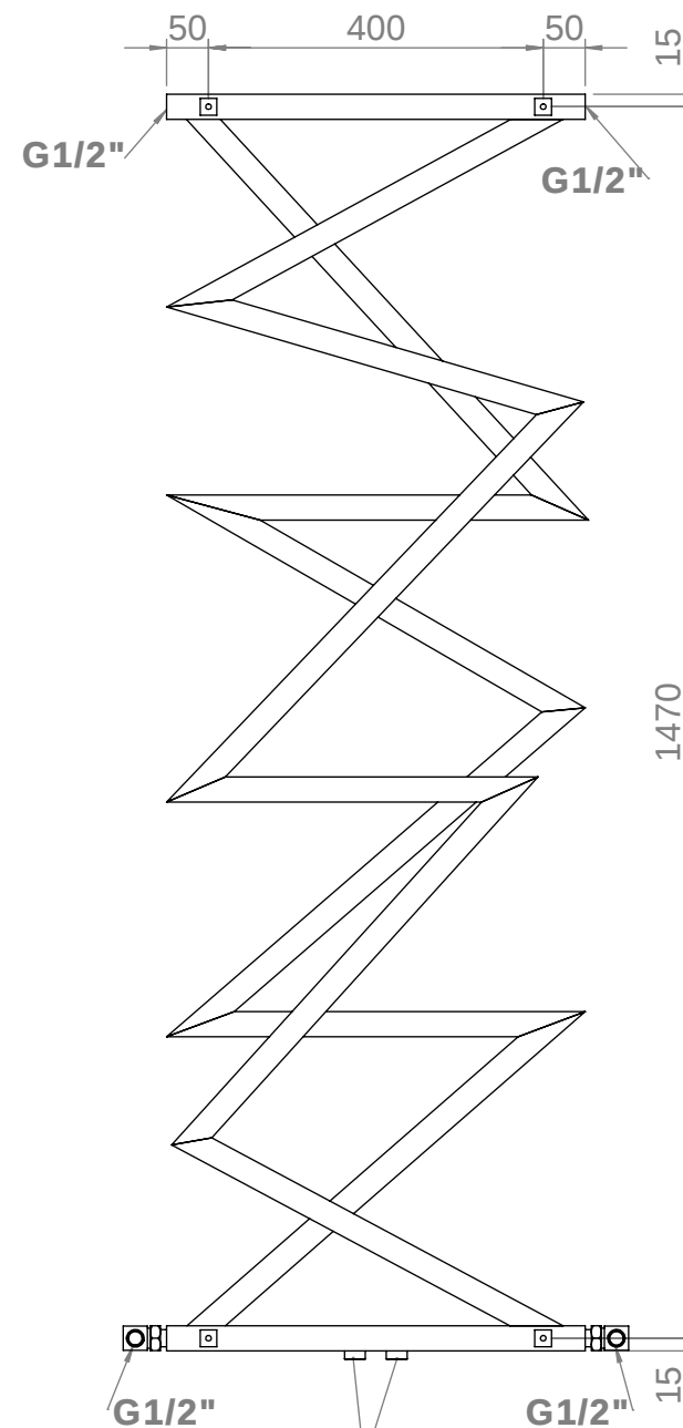
Back View
